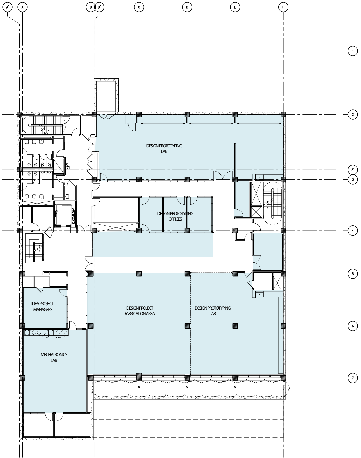
BASEMENT PLAN
